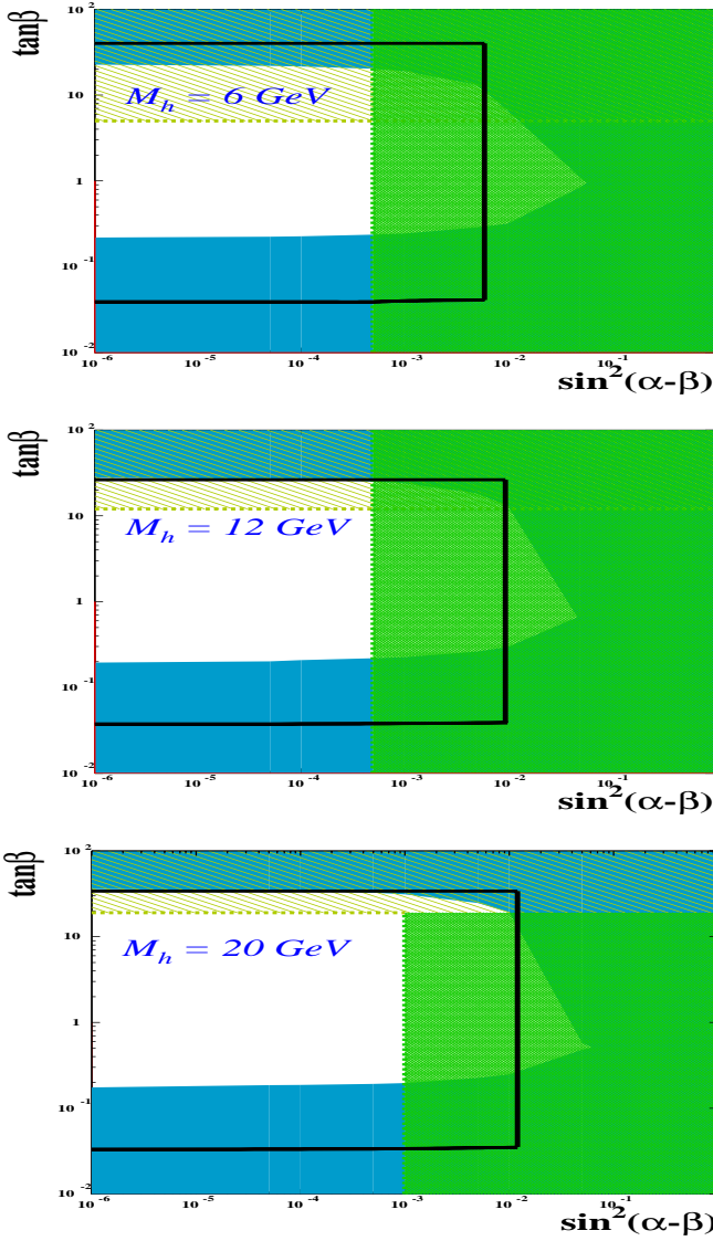
Fig. 1. Limits on \sin^2(\beta - \alpha) and \tan\beta for a light scalar h of mass M_h = 6, 12, and 20 GeV at GigaZ. The light hatched (yellow) region shows the exclusion from the Yukawa process, the cross hatched (green) region the one from Higgsstrahlung; the dark area depicts the exclusion range from Z \rightarrow \gamma h (with mass of H^\pm = 300 GeV). Also shown are the current best limits from LEP (black line)
