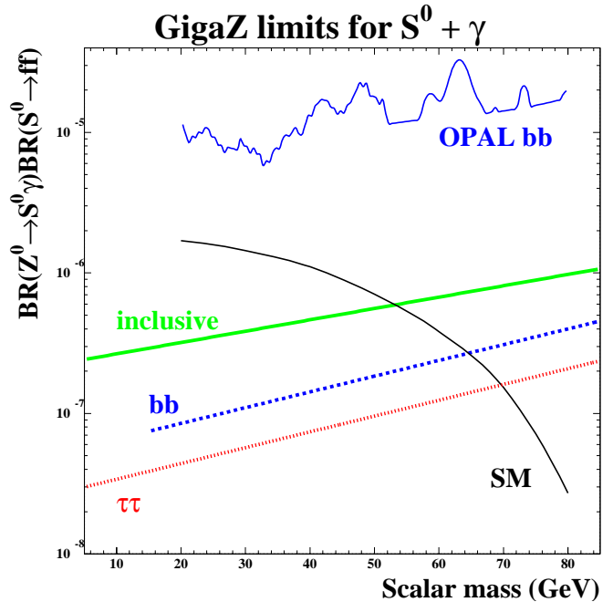
Fig. 4. Potential sensitivity on the branching ratio Z \rightarrow S + \gamma expected at GigaZ for various decay modes. The full (green) line shows the limits for decays into any kind of quarks or gluons ( inclusive ), the dashed (blue) into beauty quarks, and the dotted (red) into \tau pairs. Also indicated are the current LEP reach for decays into bottom quarks [21] (narrow full/blue line) and the standard model prediction (black line)
