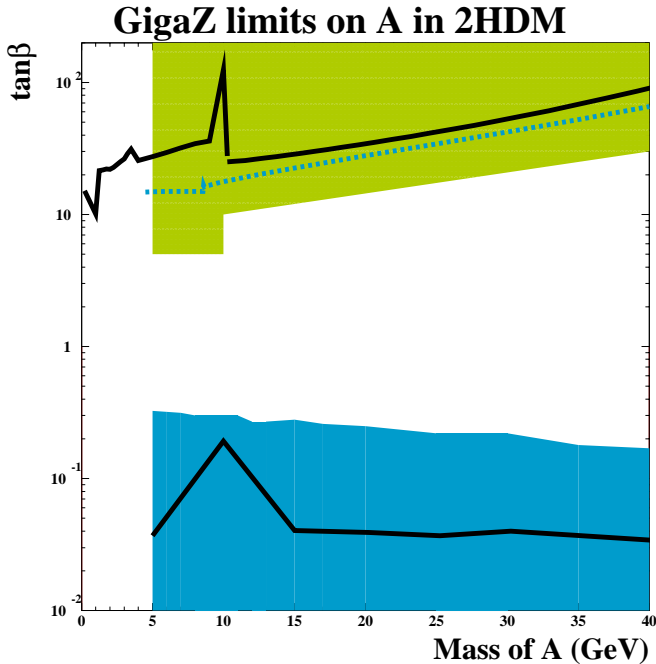
Fig. 3. Potential exclusion range at GigaZ for the light scalar A as a function of its mass and \tan\beta . The upper light (green) shaded region is excluded by the Yukawa process, the lower dark (blue) shaded region due to from Z \rightarrow A\gamma . The upper limit from Z \rightarrow A\gamma for \tan\beta > 1 is indicated by the (blue) dotted line. Also shown are the current best limits obtained at LEP (black lines, upper, from the Yukawa process and lower from the radiative Z decay)
