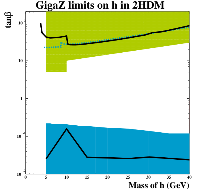
Fig. 2. Potential exclusion range at GigaZ for the light scalar h as a function of its mass and \tan\beta (for \sin(\beta - \alpha)=0 ). The upper light (green) shaded region is excluded by the Yukawa process, the lower dark (blue) shaded region due to Z \rightarrow h\gamma . The upper limit from Z \rightarrow h\gamma for \tan\beta > 1 is indicated by the (blue) dotted line. Also shown are the current best limits obtained at LEP (black lines, upper, from the Yukawa process and lower from the radiative Z decay)
